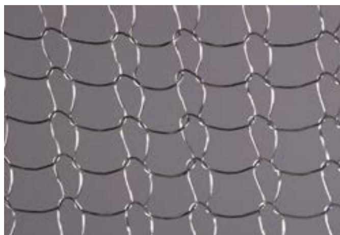
Enlarged photograph of KnitMesh's 'standard' enclosure mesh. Finish is as-knit 304 stainless steel.
